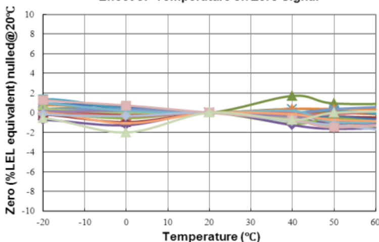
Effect of Temperature on Zero Signal
