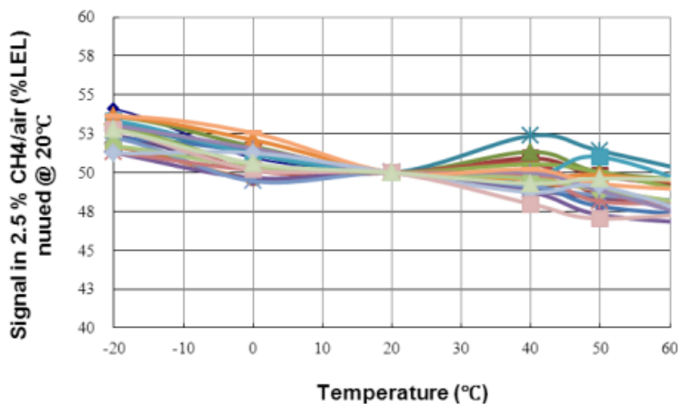
Effect of Temperature on Methane Signal
