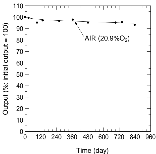
Fig 1 Long-term stability
