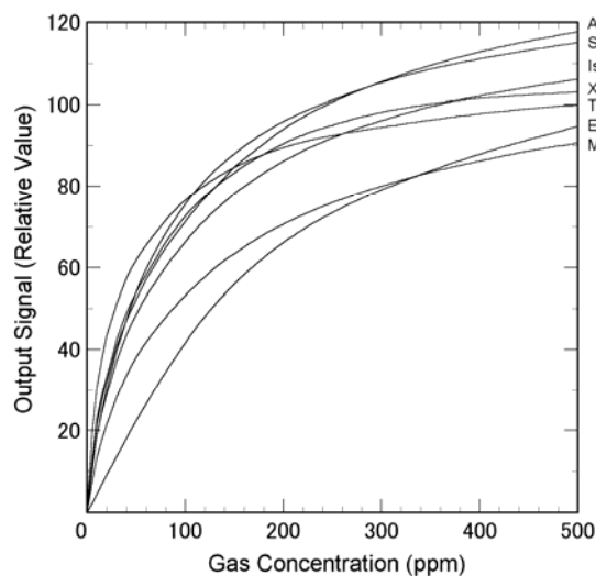
Fig 1 Sensitivity characteristic
