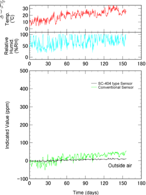
Fig 2 Long-term stability on field
