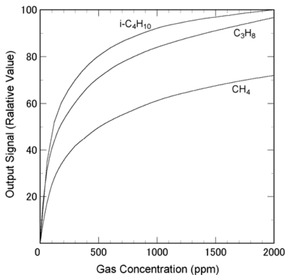
Fig 1 Sensitivity characteristic
