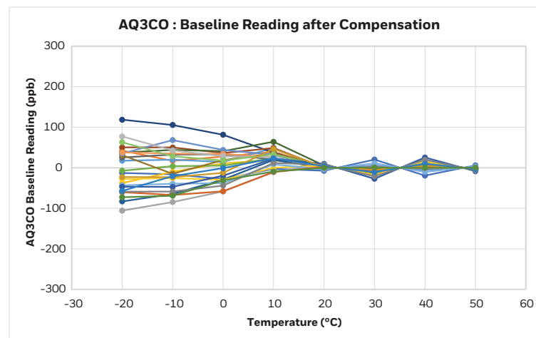
Figure 7. Baseline vs Temperature after Compensation
