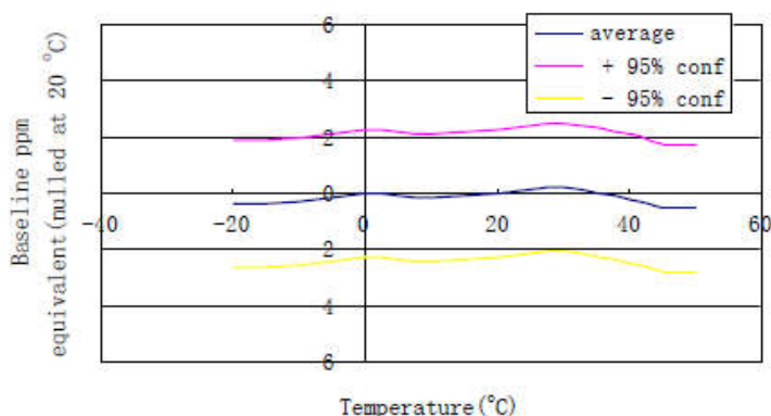
3CO-500-Sensitivity temperature dependence
