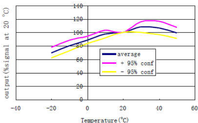
3CO-500-Sensitivity temperature dependence
